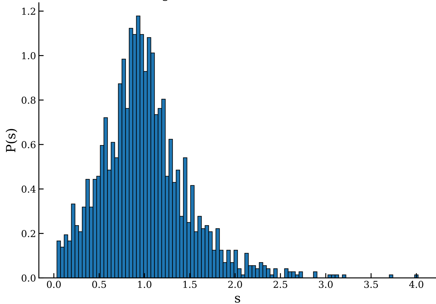
Range chain R=2 \langle r \rangle = 0.6035
